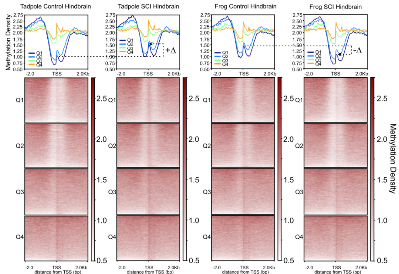
Fig. 4 Degree of CpG methylation surrounding the transcriptional start site (TSS; \pm 2.0 kb) correlated with RNA expression for regenerative (tadpole) and non regenerative (frog) hindbrain before and after SCI. Top , average level of CpG methylation for different levels of gene expression (Q1 to Q4, representing the 25% most highly to least expressed genes, respectively from a total of 45,099 gene models in X. laevis v.9.1 [122]). (+ or - \Delta , indicates the injury-induced changes for genes in Q1. x-axis units, distance from the predicted transcription start site (TSS) in kilobases (kb); y-axis units (Methylation Density), number of 5mCs in a 50 bp bin \times 1 million/total number of Cs. Bottom , heatmaps of CpG methylation for each quartile, clustered from highest to lowest. The degree of CpG-methylation exhibited the expected negative correlation with RNA expression, but for the top two quartiles, it increased in regenerative hindbrain and decreased in non-regenerative hindbrain after SCI. The degree of CpG methylation is indicated by the intensity of the color, as indicated to the right of each heatmap (Methylation Density)
